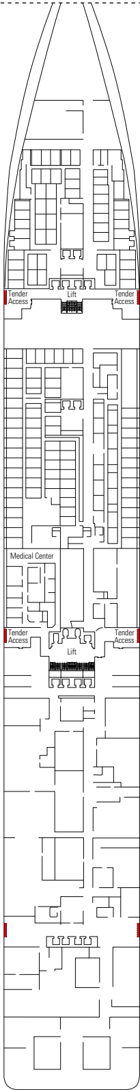
DECK 4 AMBRA
